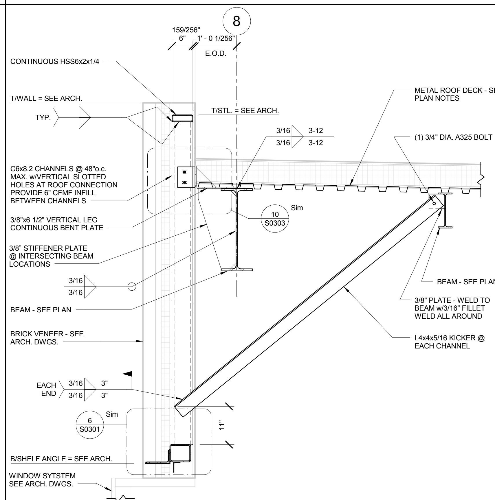
10 FRAMING SECTION 3/4" = 1'-0"
