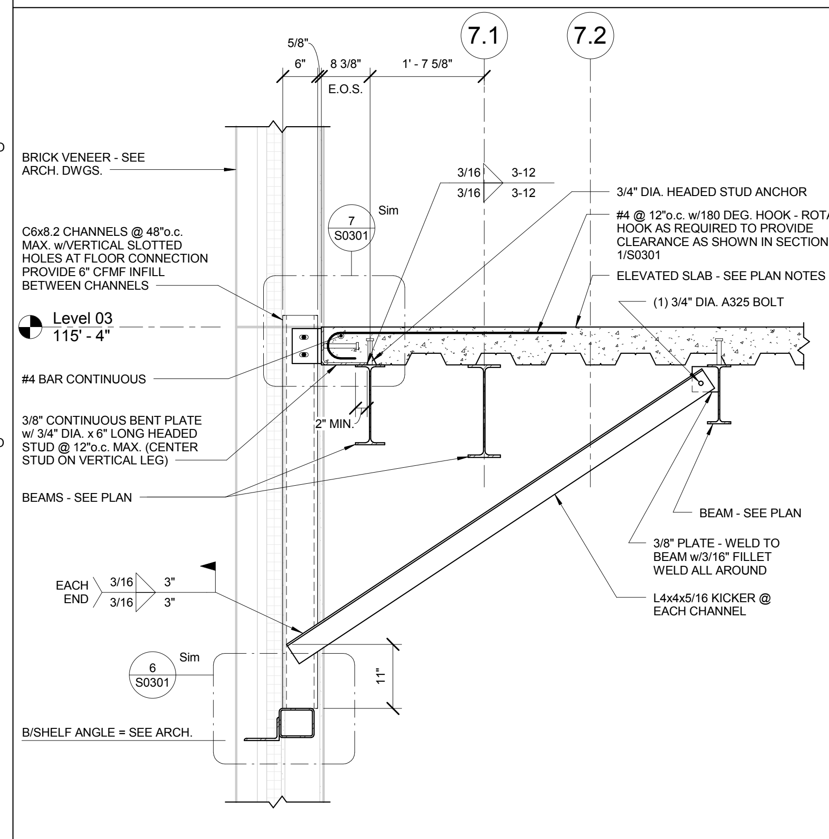
12 FRAMING SECTION 3/4" = 1'-0"
