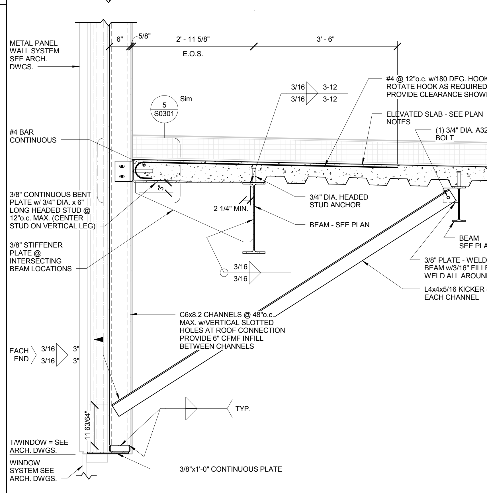
11 FRAMING SECTION 3/4" = 1'-0"
