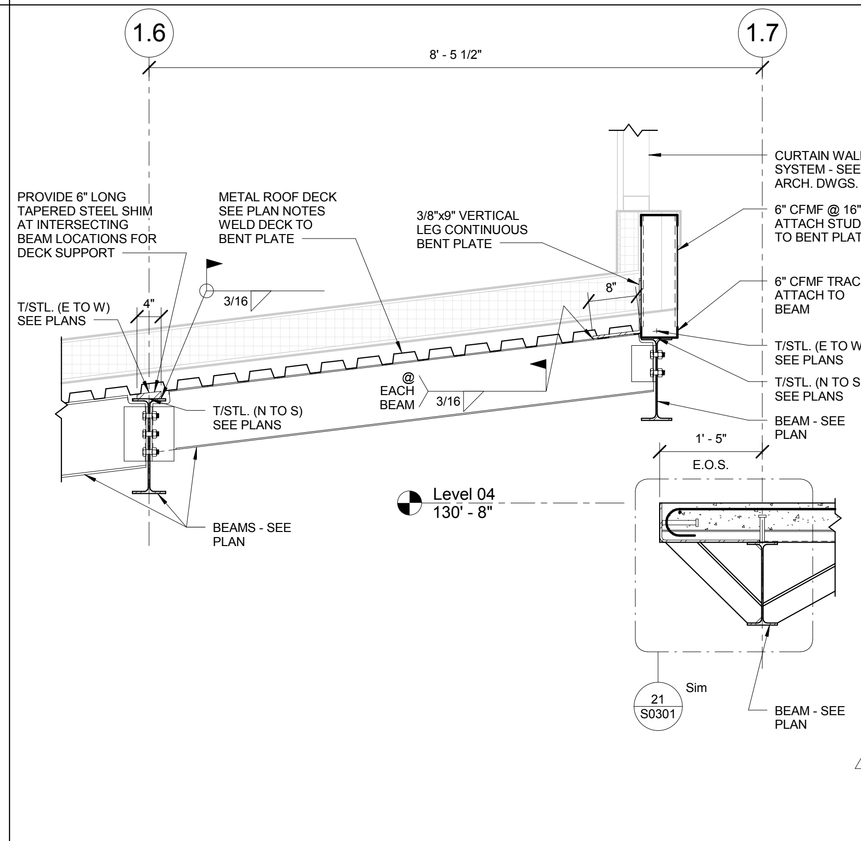
6 FRAMING SECTION 3/4" = 1'-0"
