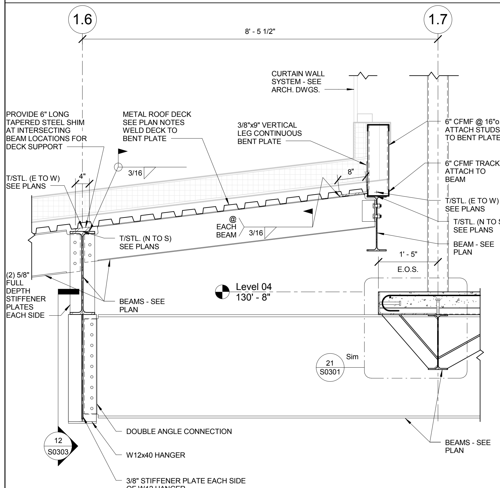
5 FRAMING SECTION 3/4" = 1'-0"
