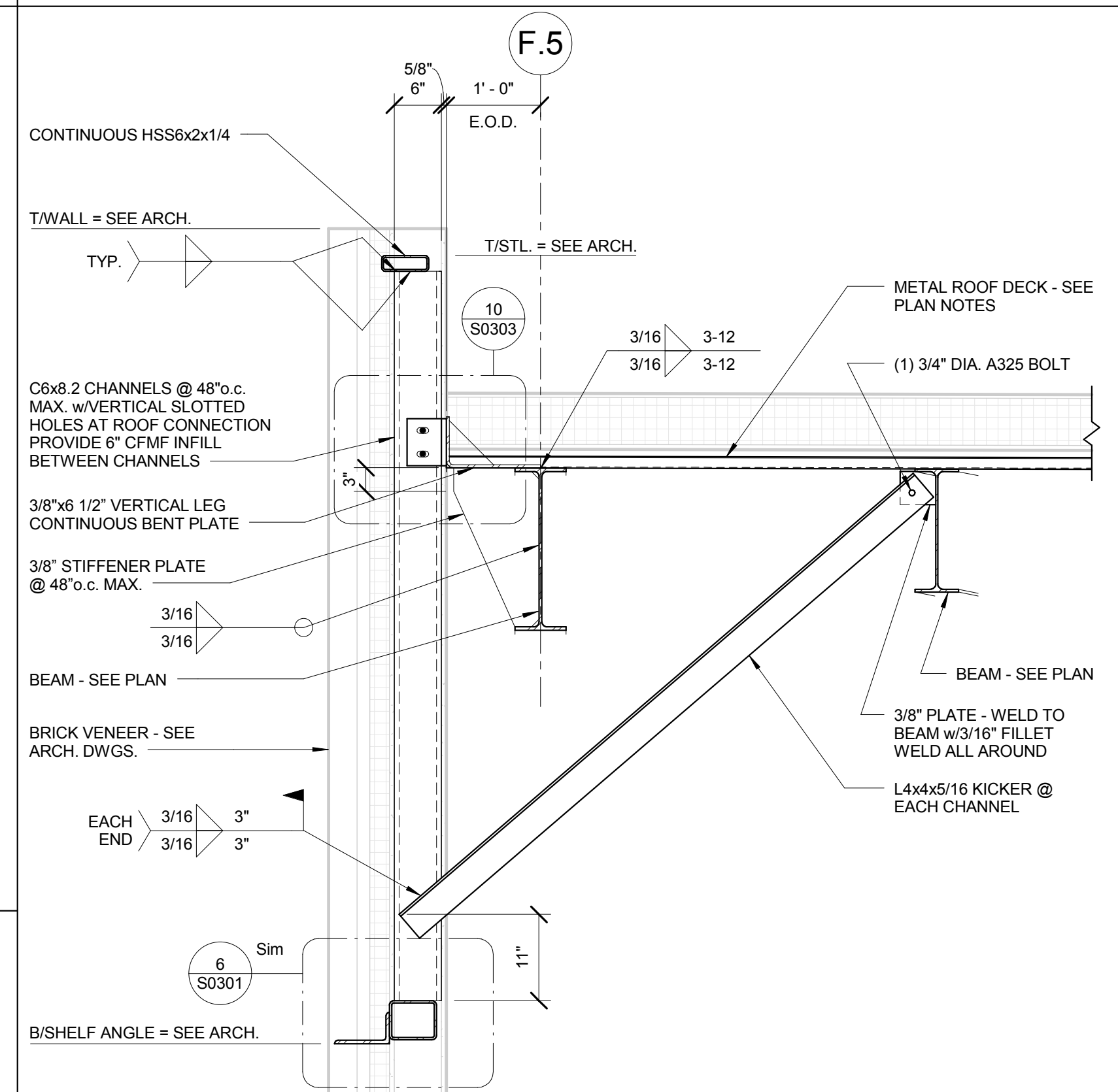
8 FRAMING SECTION 3/4" = 1'-0"
