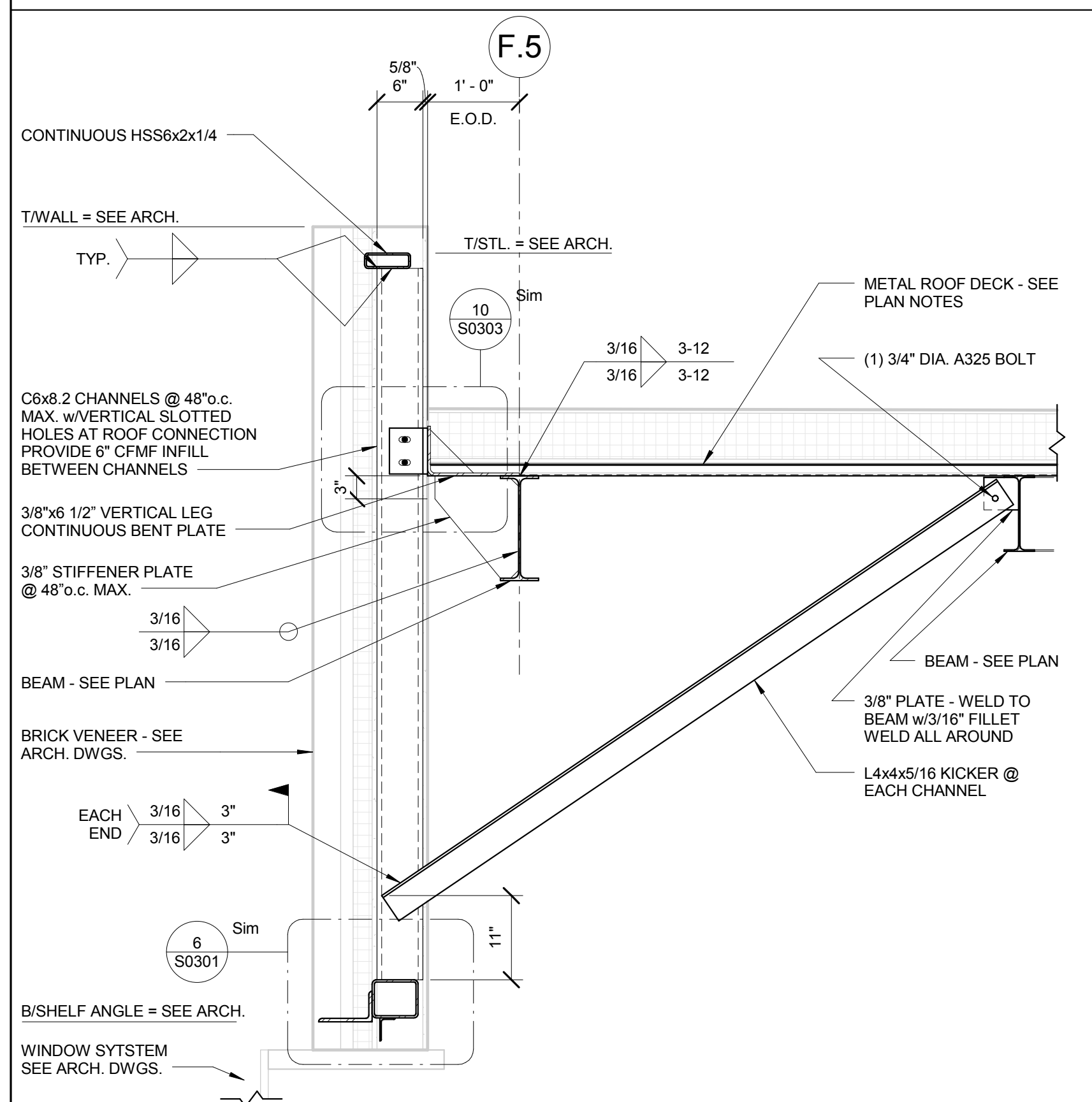
9 FRAMING SECTION 3/4" = 1'-0"
