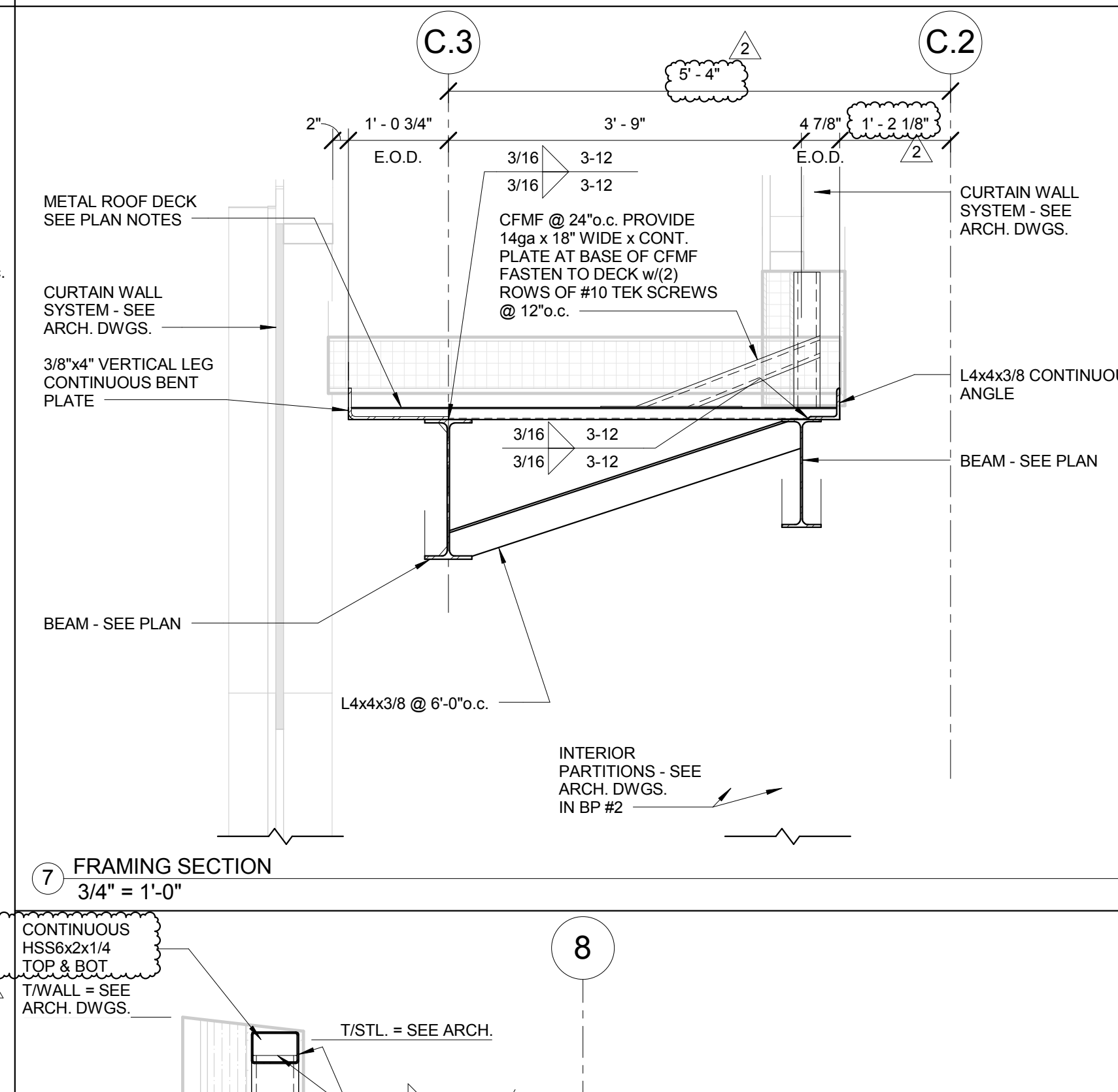
7 FRAMING SECTION 3/4" = 1'-0"
